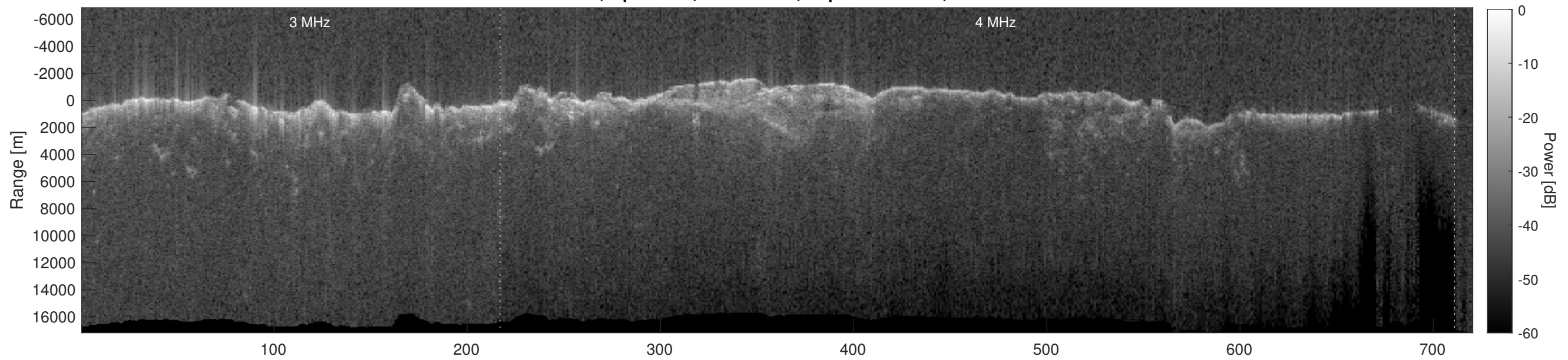
Orbit 6546, Depth-Corrected Cluttergram
