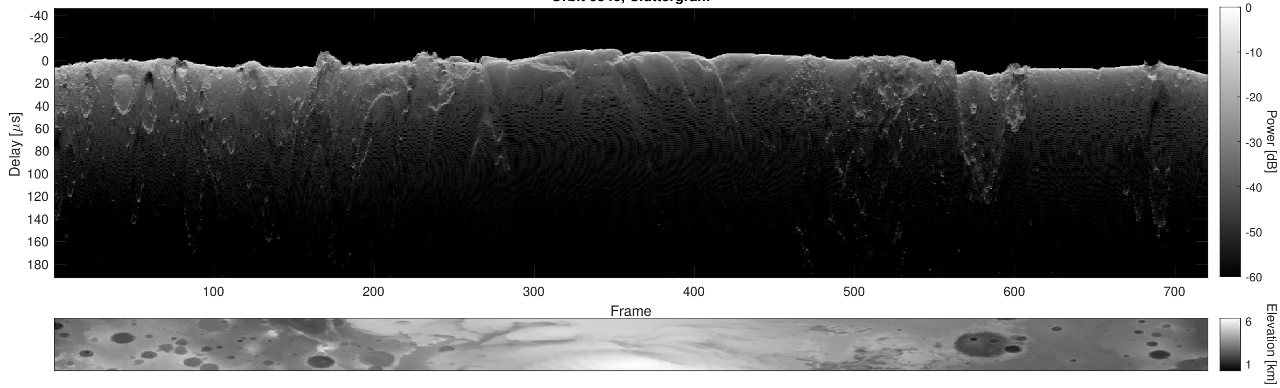
Orbit 6546, Cluttergram
