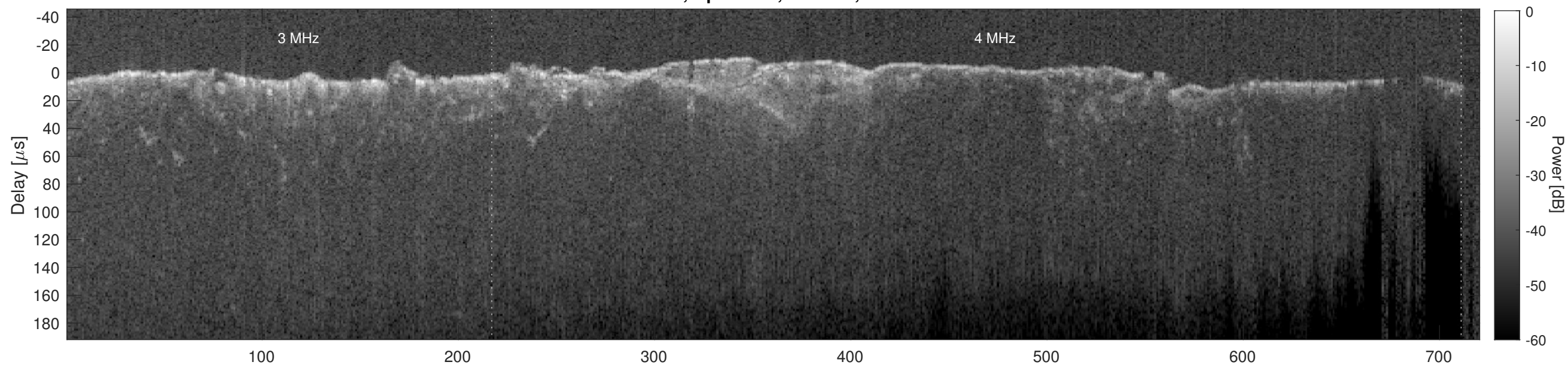
Orbit 6546, Cluttergram
