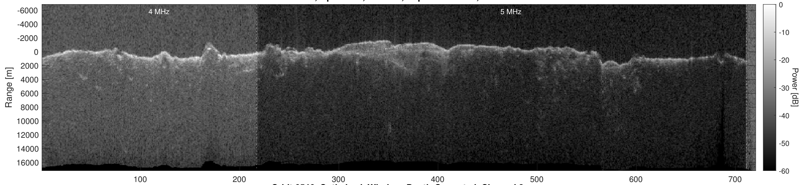
Orbit 6546, Optimized, Window, Depth-Corrected, Channel 2
