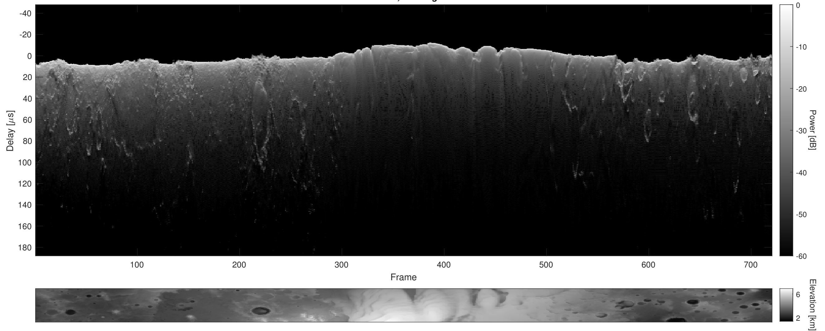
Orbit 6547, Cluttergram
