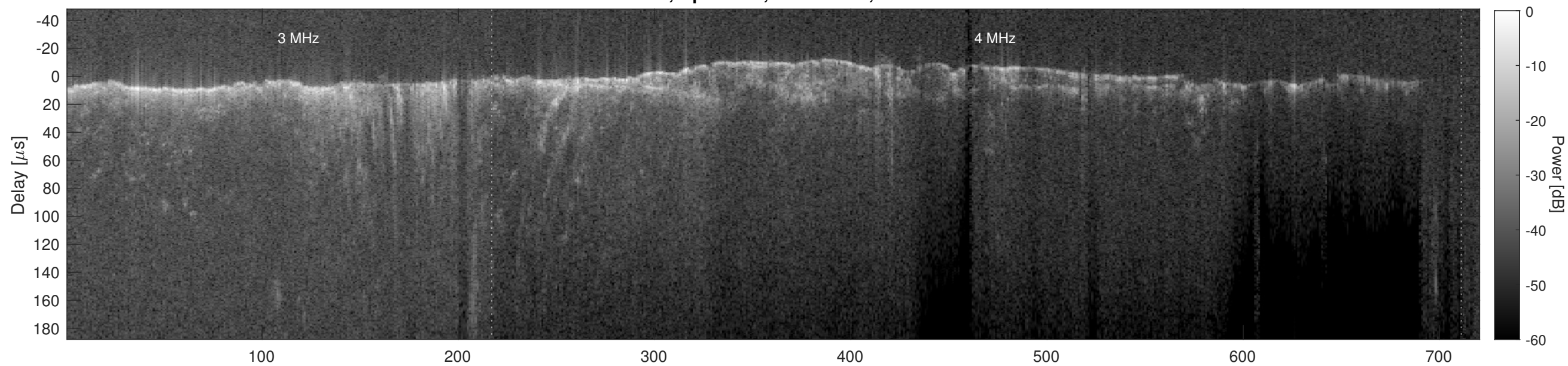
Orbit 6547, Cluttergram
