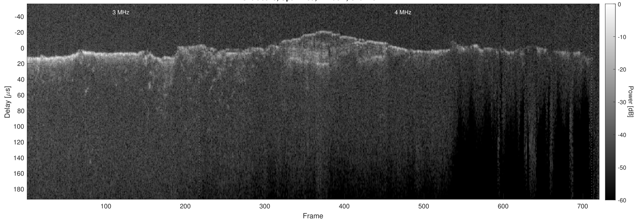
Orbit 6548, Optimized, Window, Channel 2
