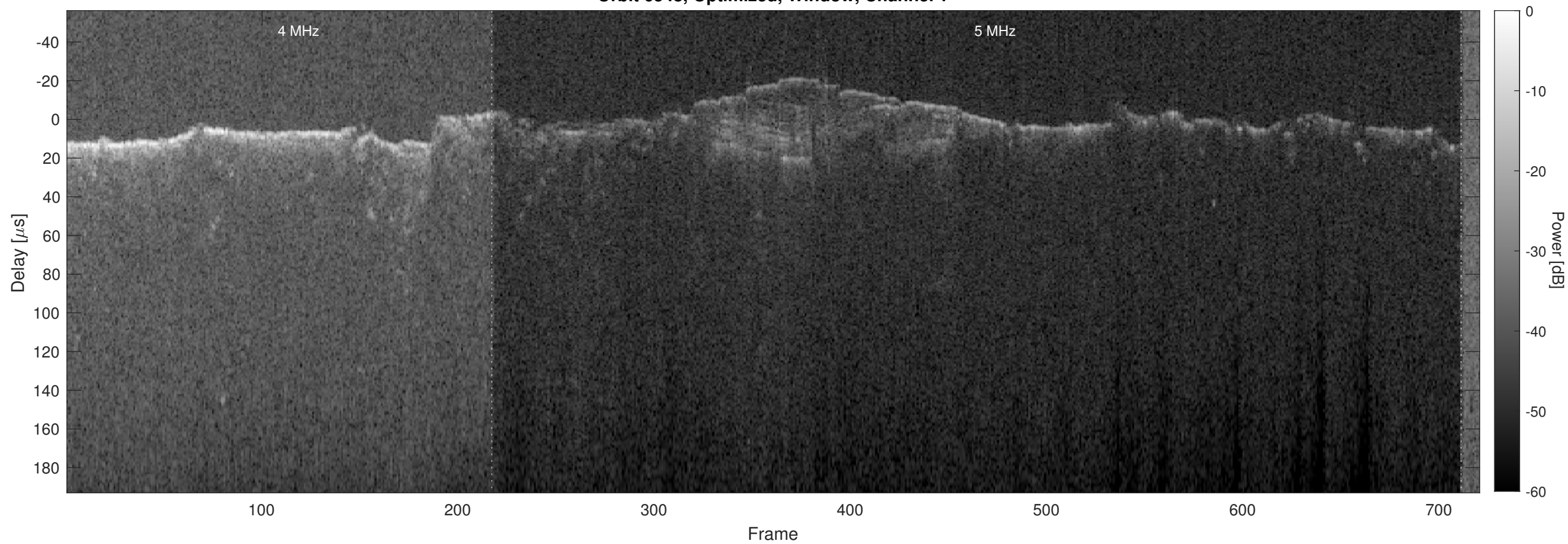
Orbit 6548, Optimized, Window, Channel 2
