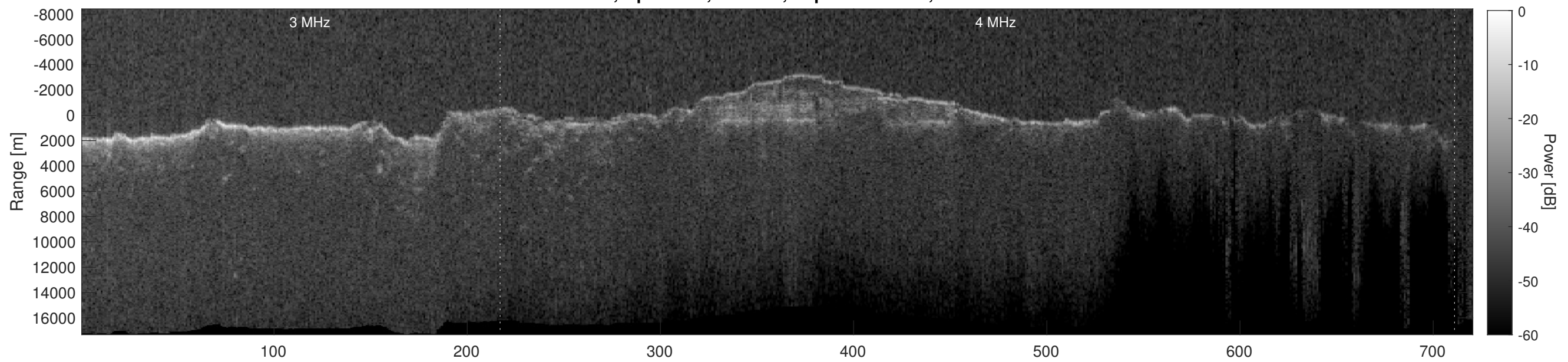
Orbit 6548, Depth-Corrected Cluttergram
