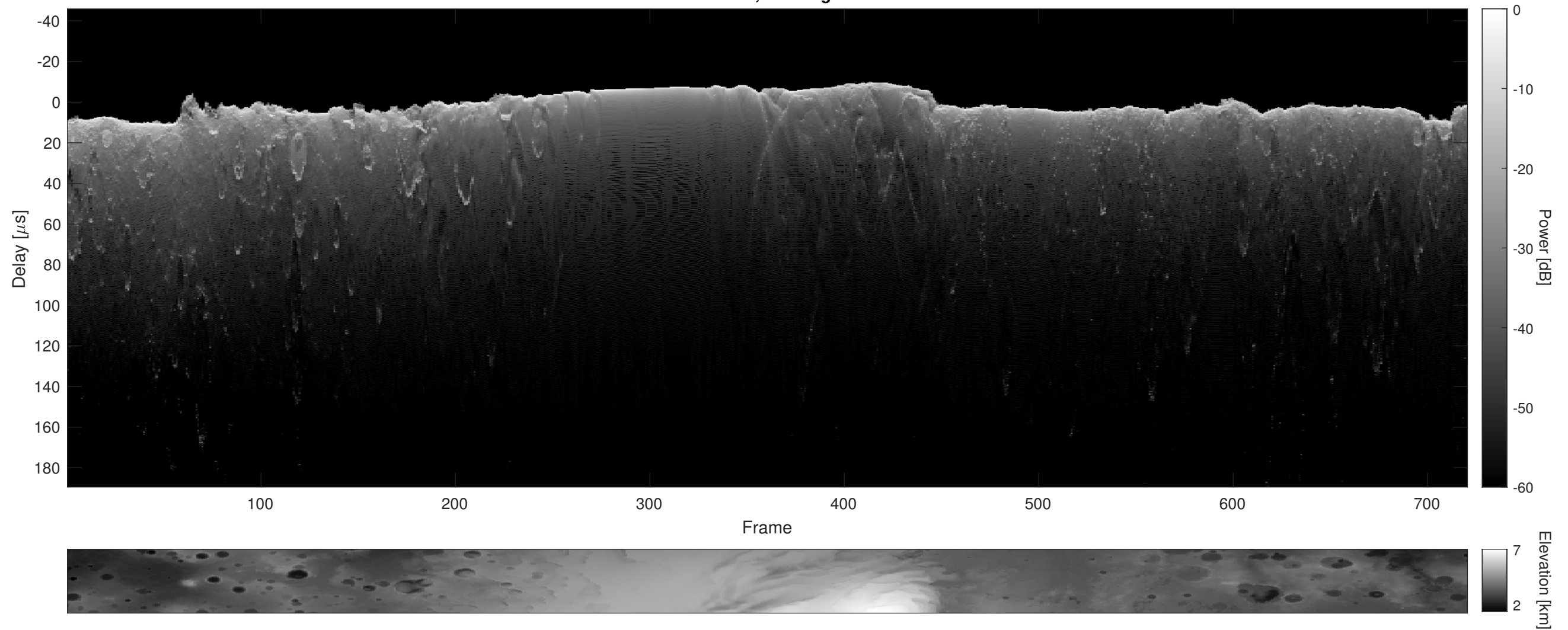
Orbit 6549, Cluttergram
