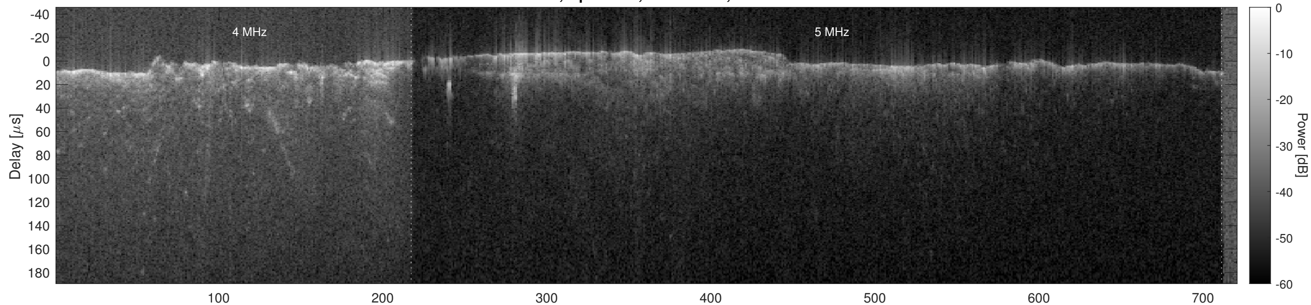
Orbit 6549, Optimized, No Window, Channel 2
