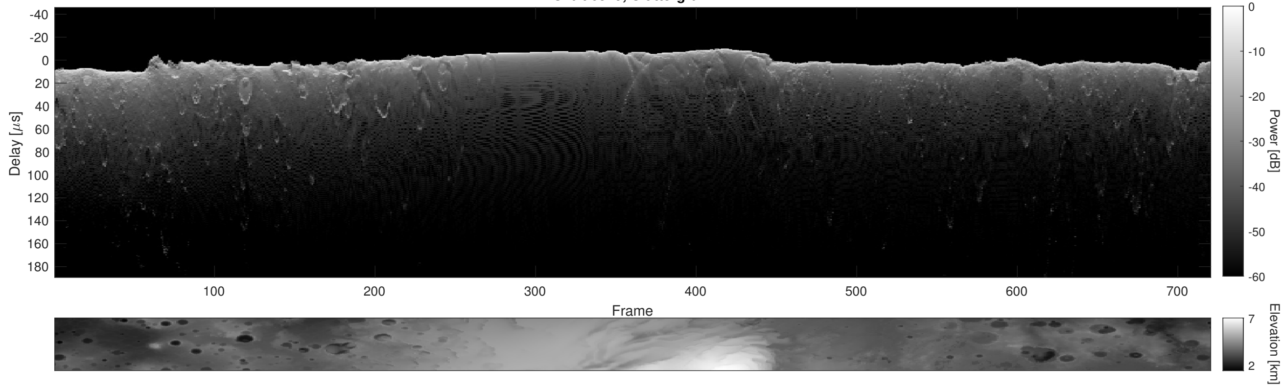
Orbit 6549, Cluttergram
