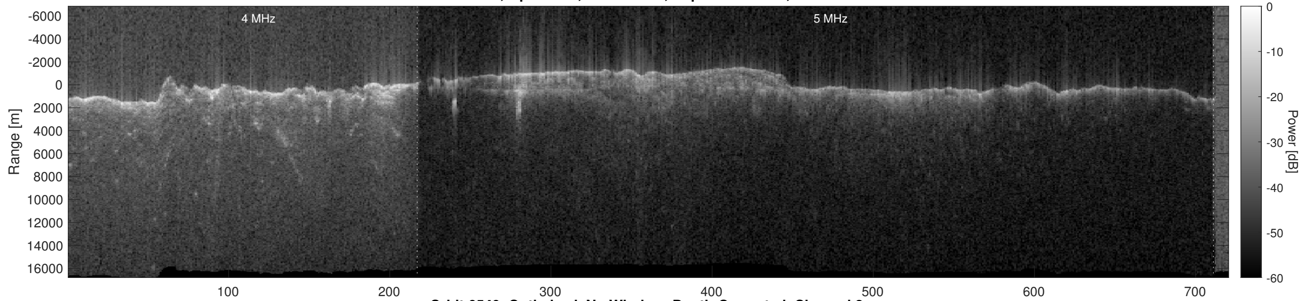
Orbit 6549, Optimized, No Window, Depth-Corrected, Channel 2
