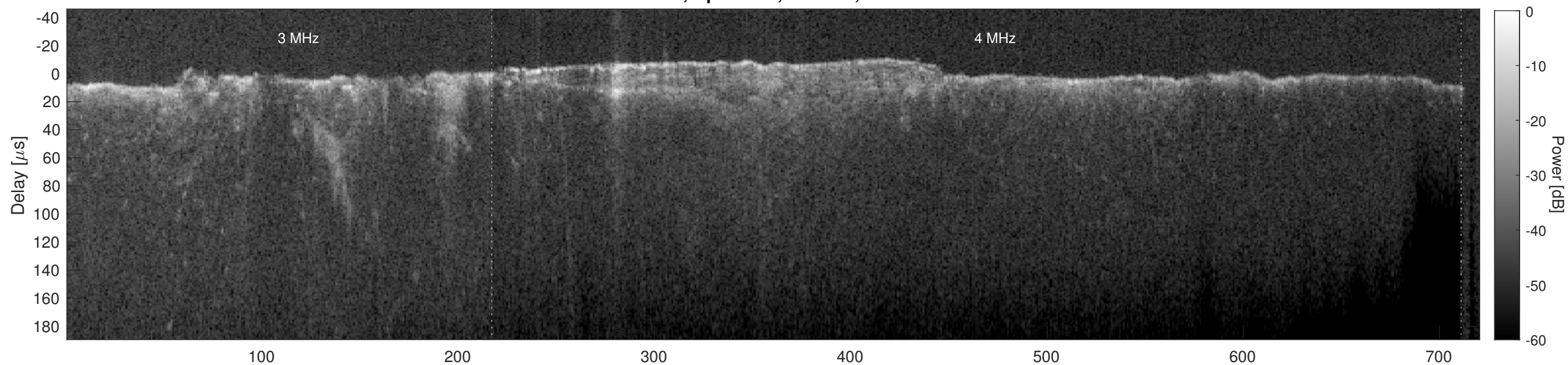
Orbit 6549, Cluttergram
