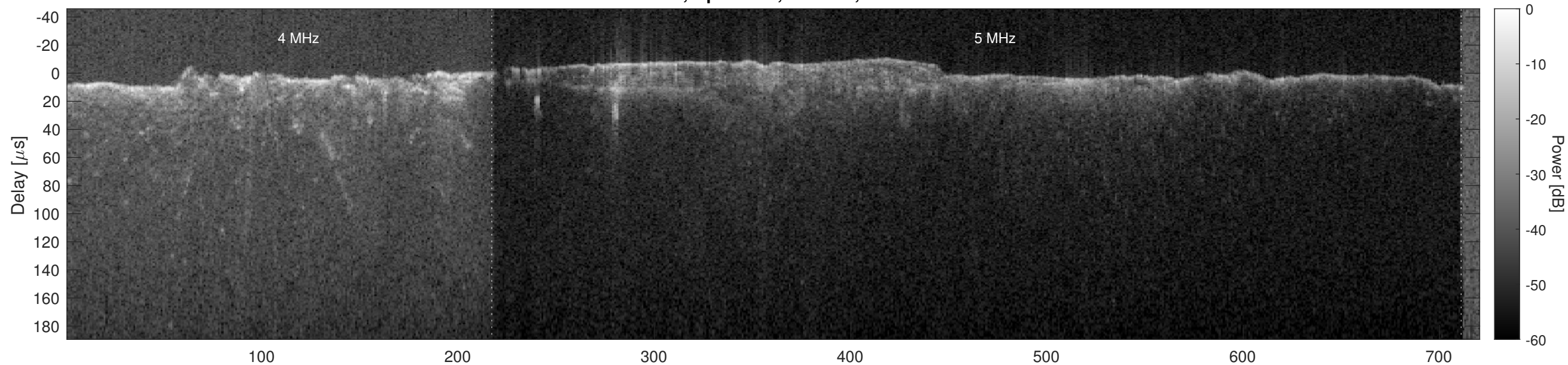
Orbit 6549, Optimized, Window, Channel 2
