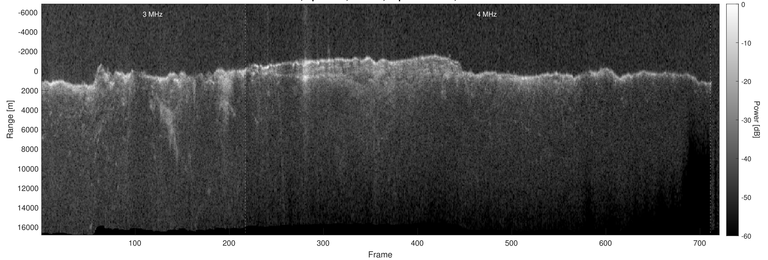
Orbit 6549, Optimized, Window, Depth-Corrected, Channel 2
