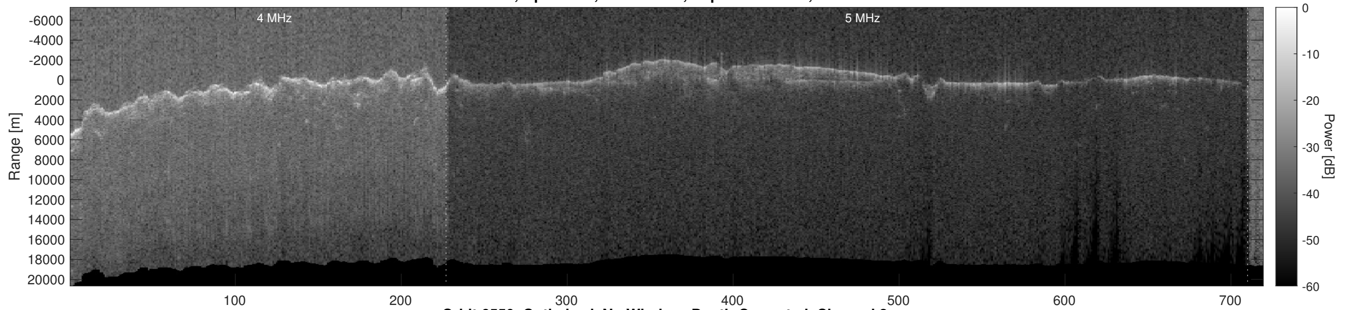
Orbit 6550, Optimized, No Window, Depth-Corrected, Channel 2
