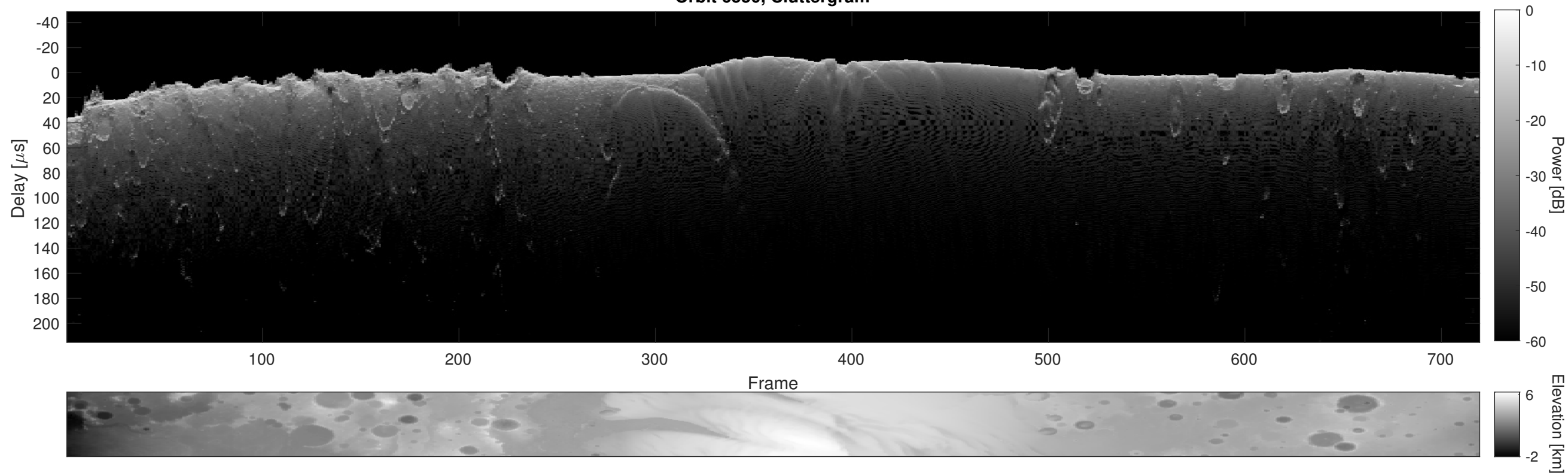
Orbit 6550, Cluttergram
