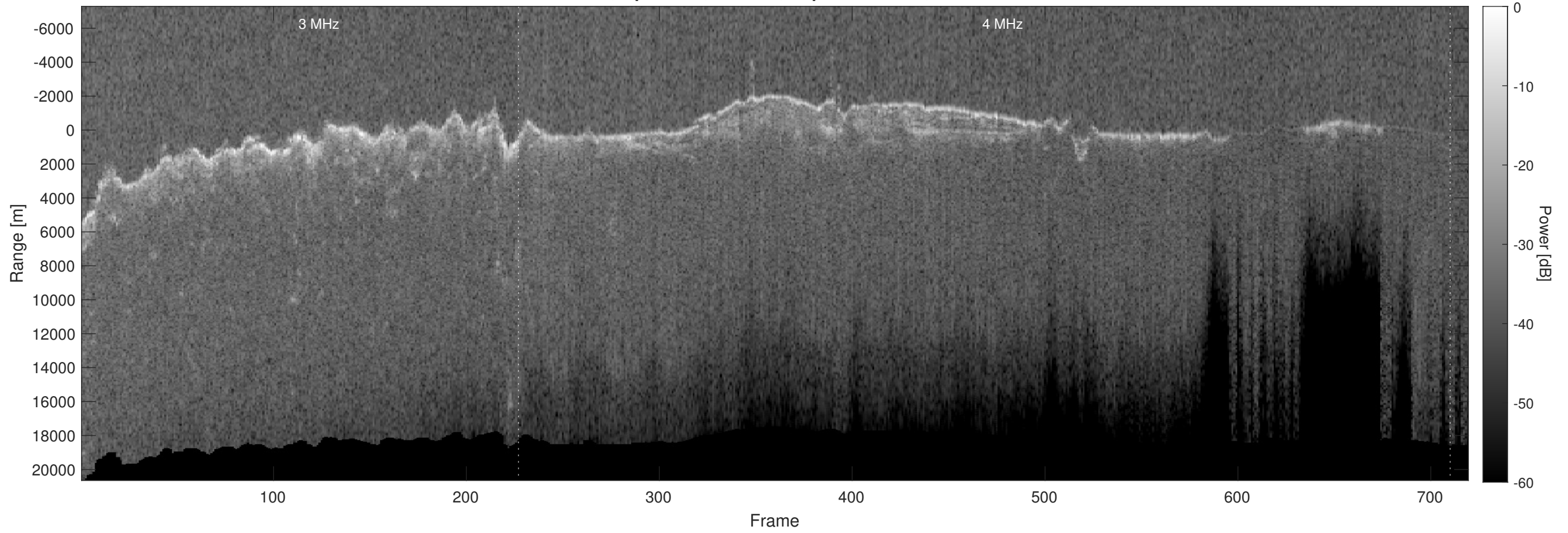
Orbit 6550, Optimized, Window, Depth-Corrected, Channel 2
