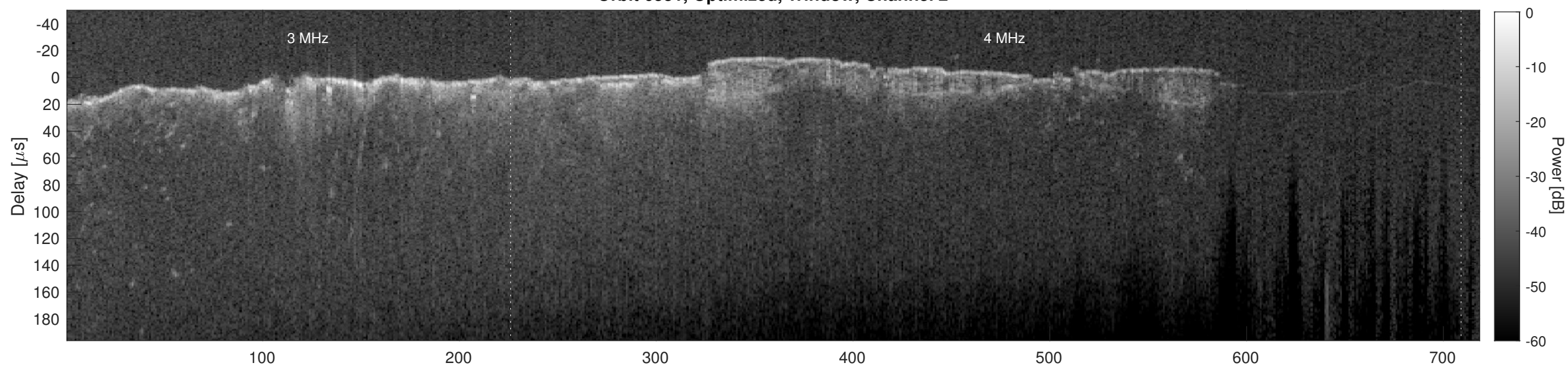
Orbit 6551, Cluttergram
