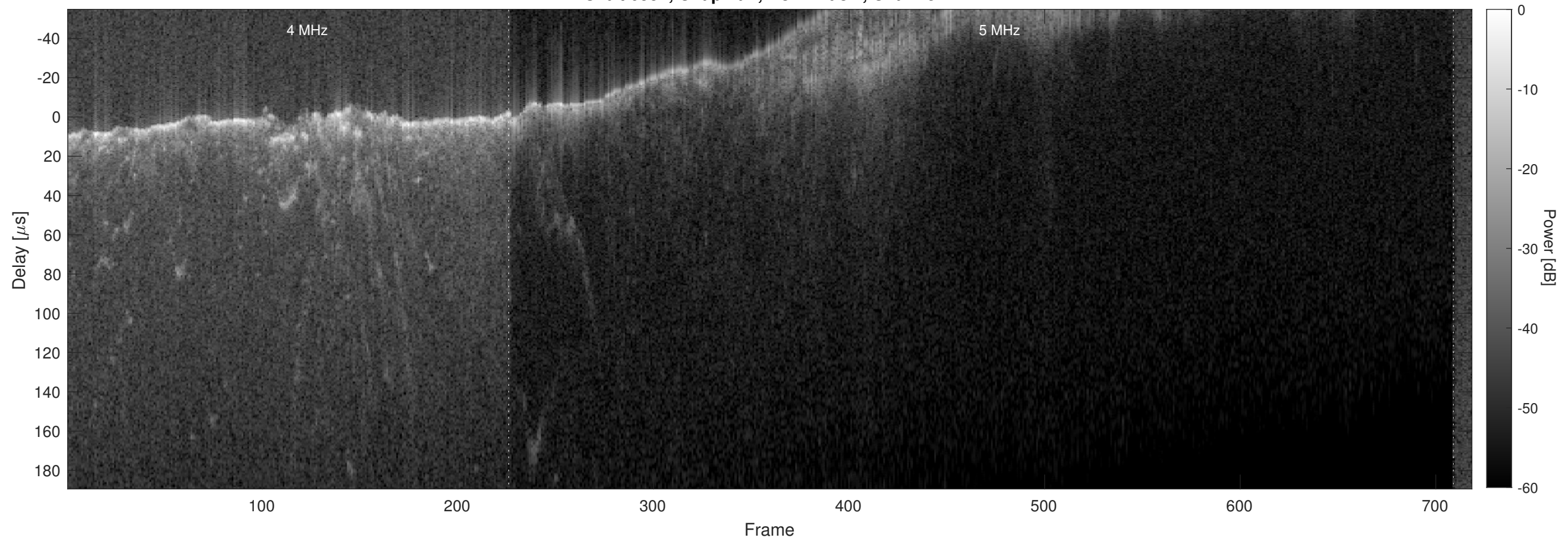
Orbit 6552, Chapman, No Window, Channel 2
