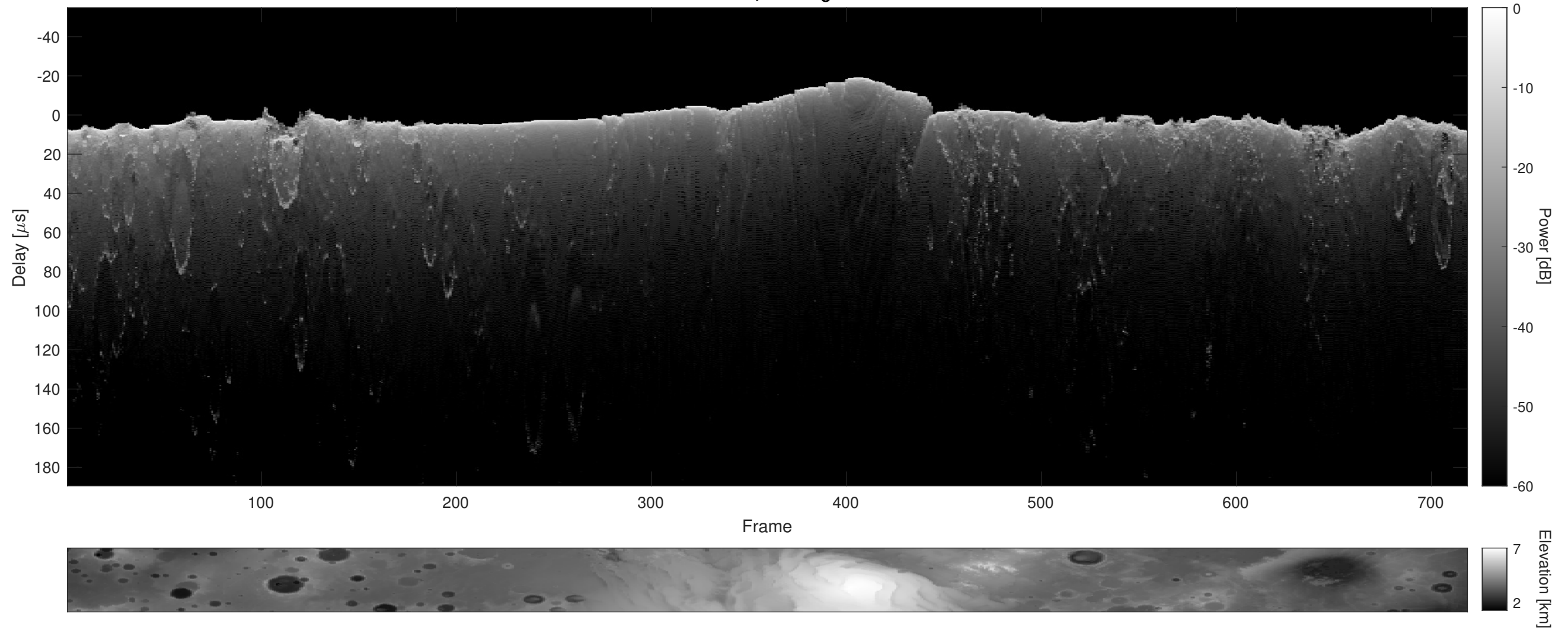
Orbit 6552, Cluttergram
