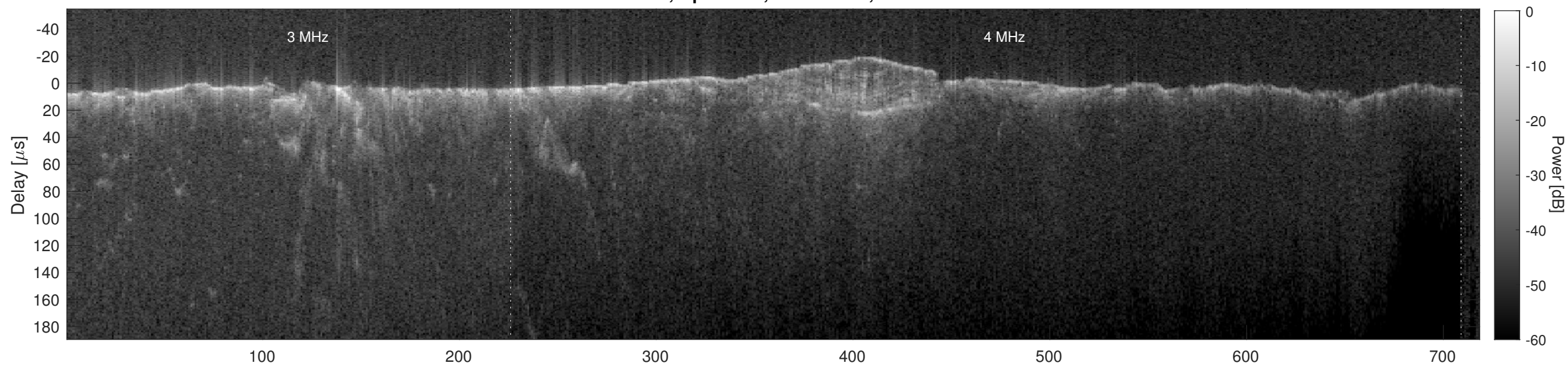
Orbit 6552, Cluttergram
