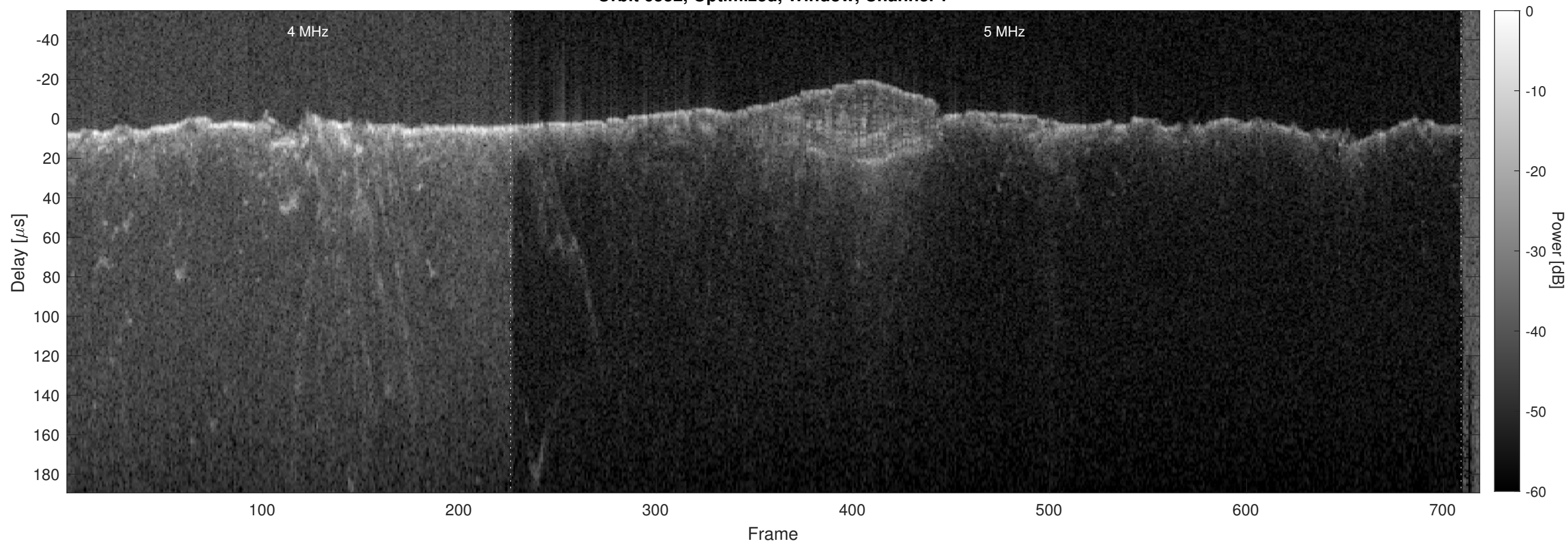
Orbit 6552, Optimized, Window, Channel 2
