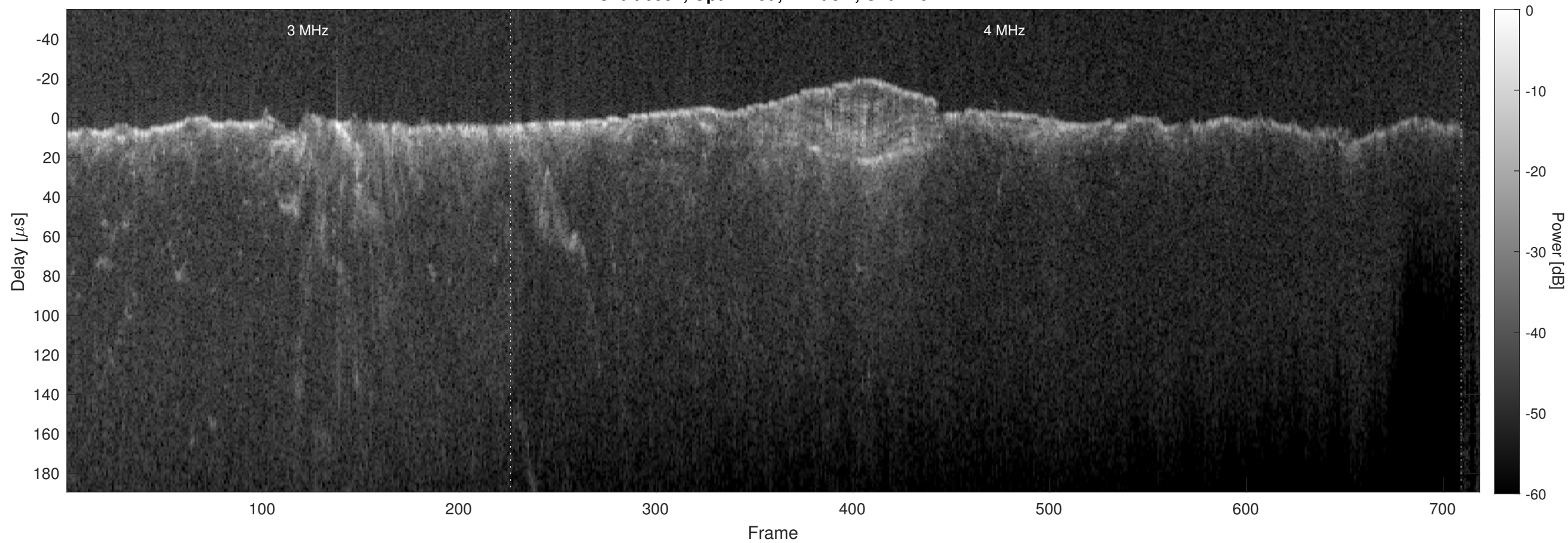
Orbit 6552, Optimized, Window, Channel 2
