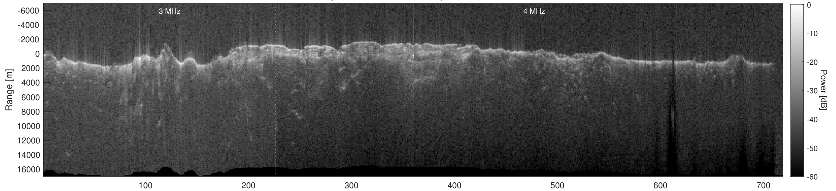
Orbit 6553, Depth-Corrected Cluttergram
