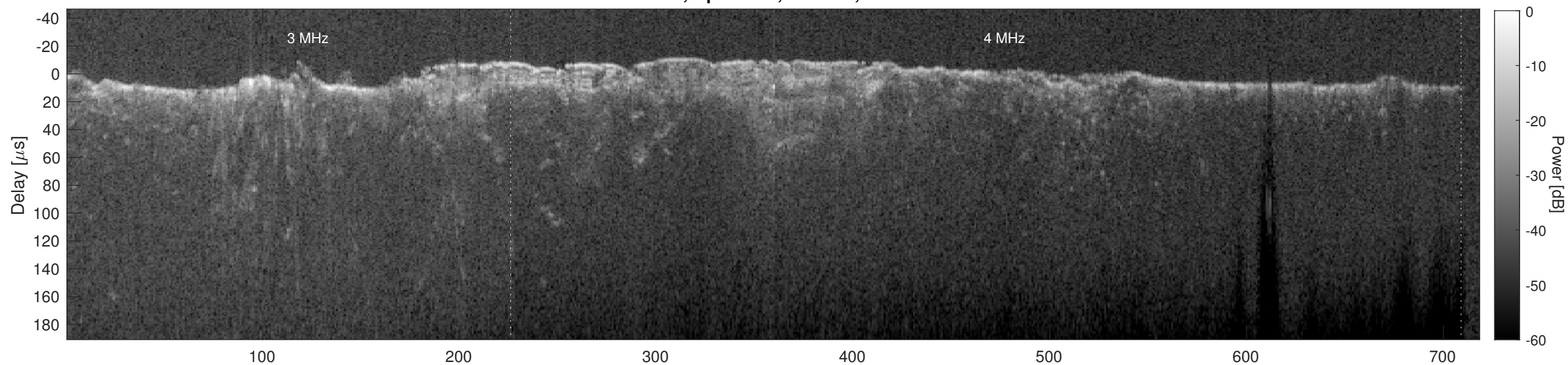
Orbit 6553, Cluttergram
