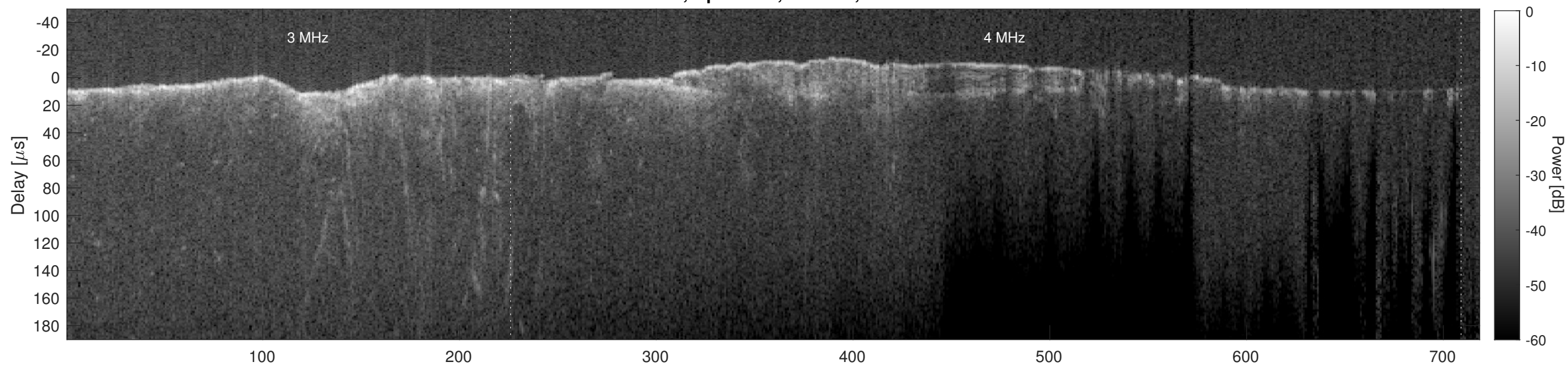
Orbit 6554, Cluttergram
