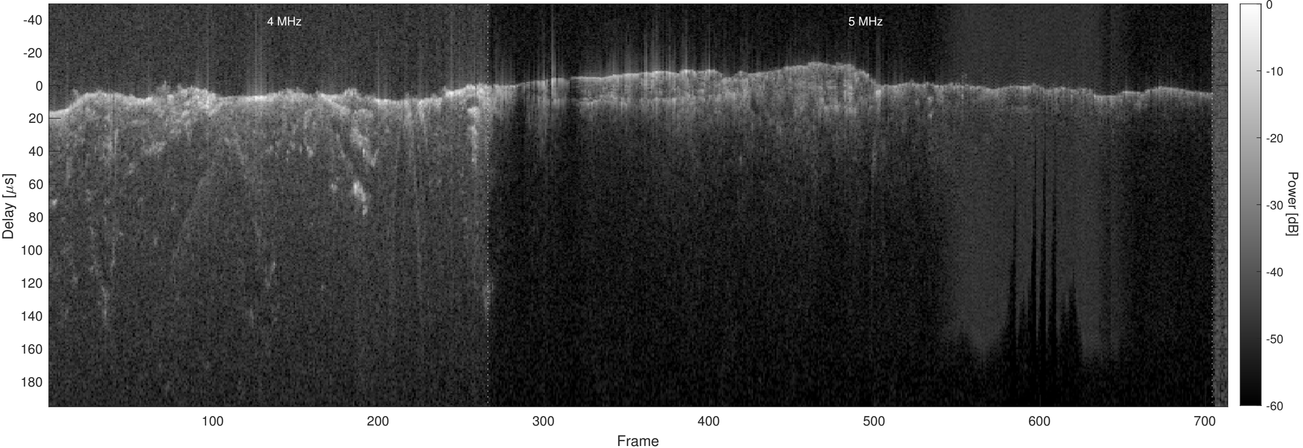
Orbit 6581, Optimized, No Window, Channel 2
