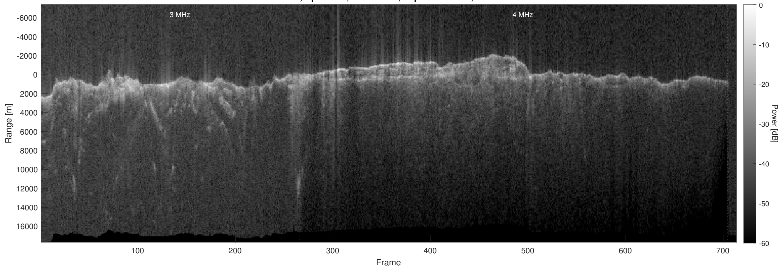
Orbit 6581, Optimized, No Window, Depth-Corrected, Channel 2
