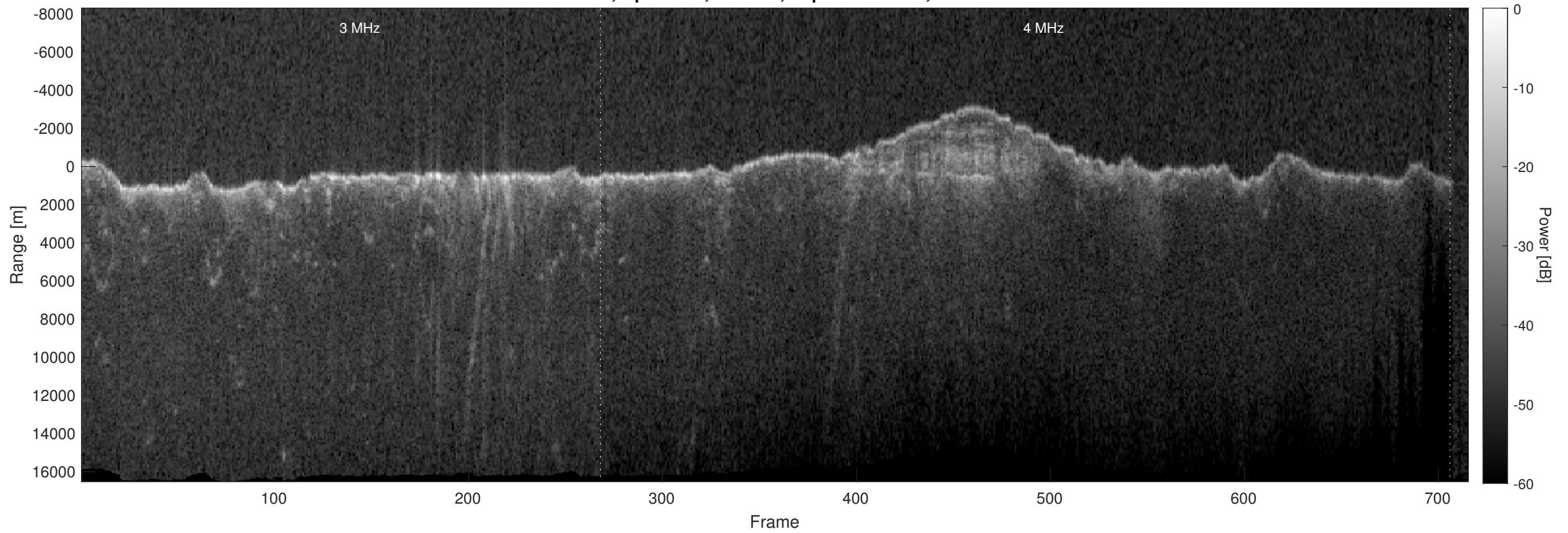
Orbit 6584, Optimized, Window, Depth-Corrected, Channel 2
