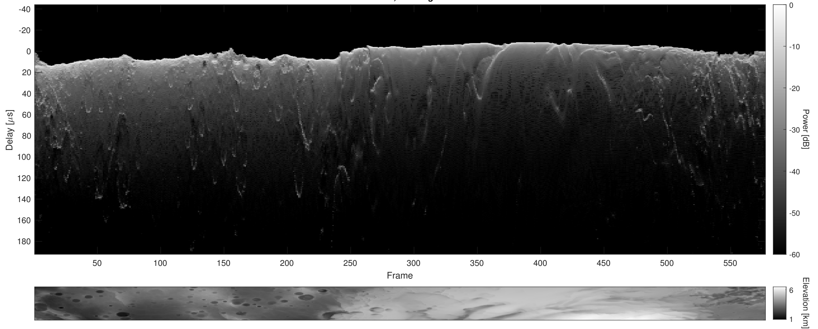
Orbit 6585, Cluttergram
