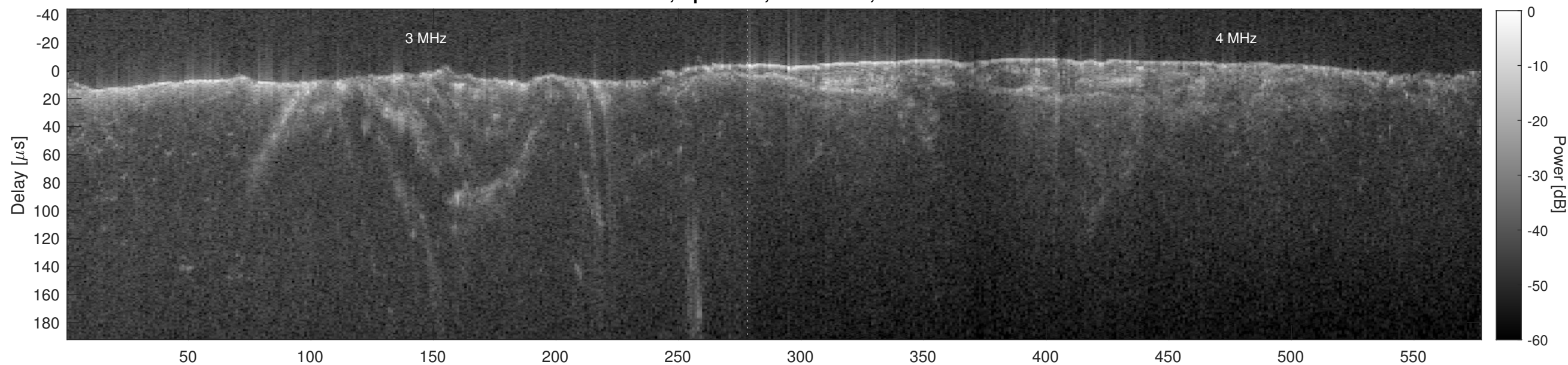
Orbit 6585, Cluttergram
