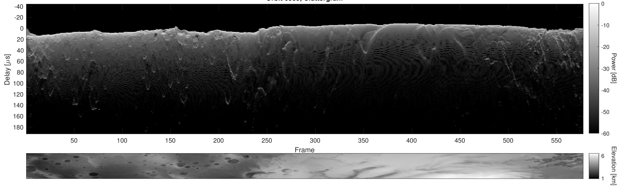
Orbit 6585, Cluttergram
