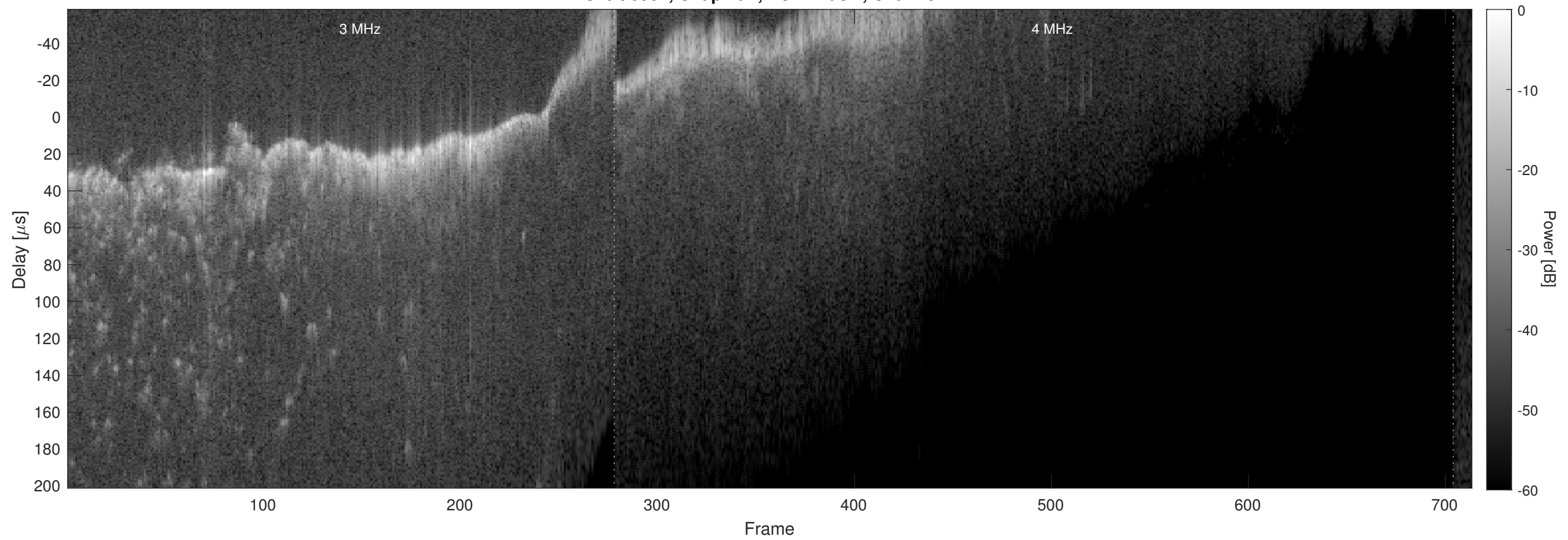
Orbit 6587, Chapman, No Window, Channel 2
