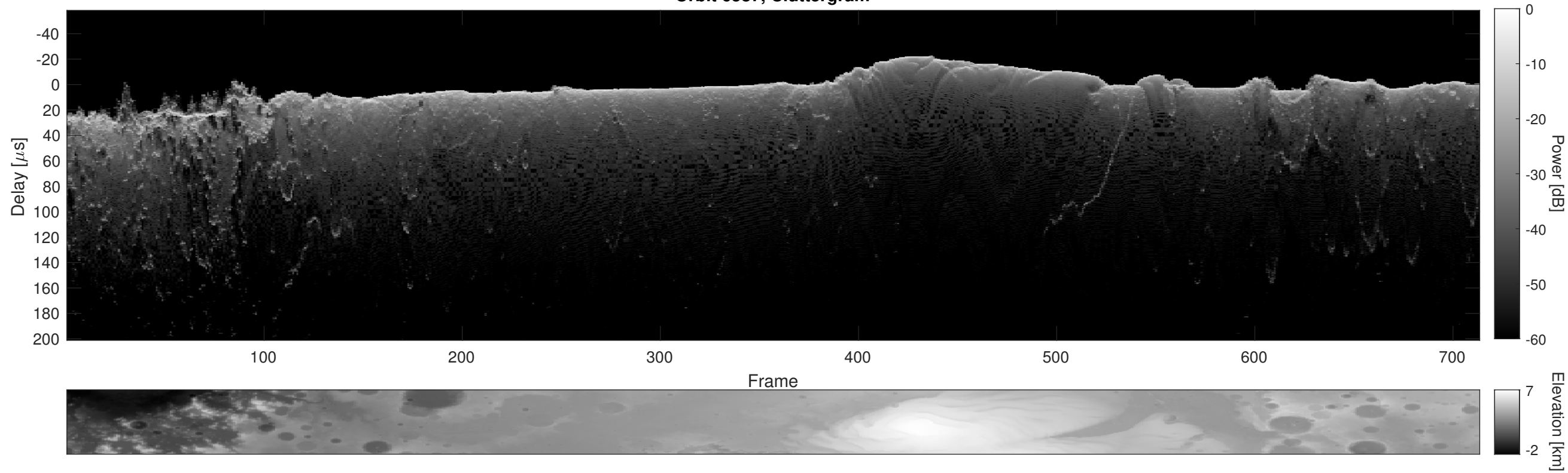
Orbit 6587, Cluttergram
