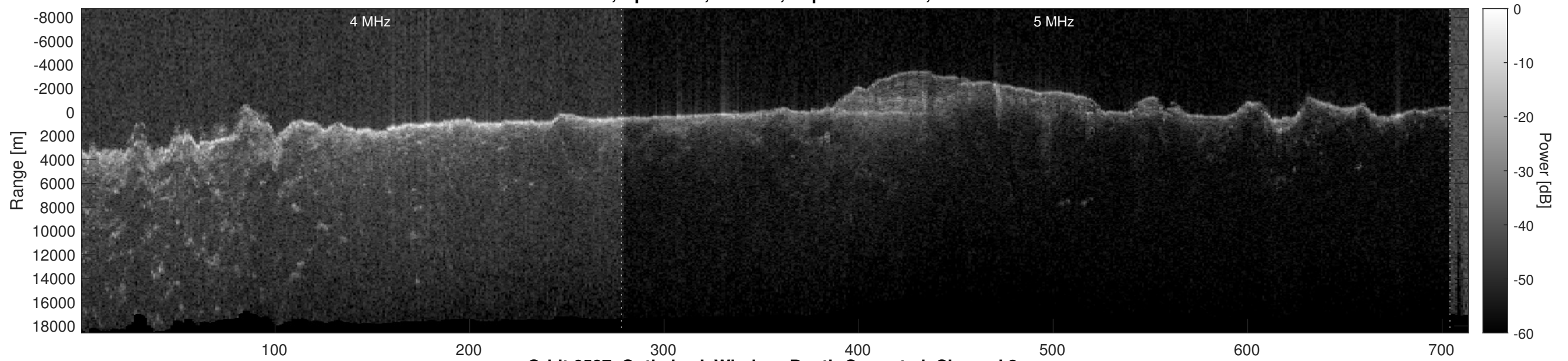
Orbit 6587, Optimized, Window, Depth-Corrected, Channel 2
