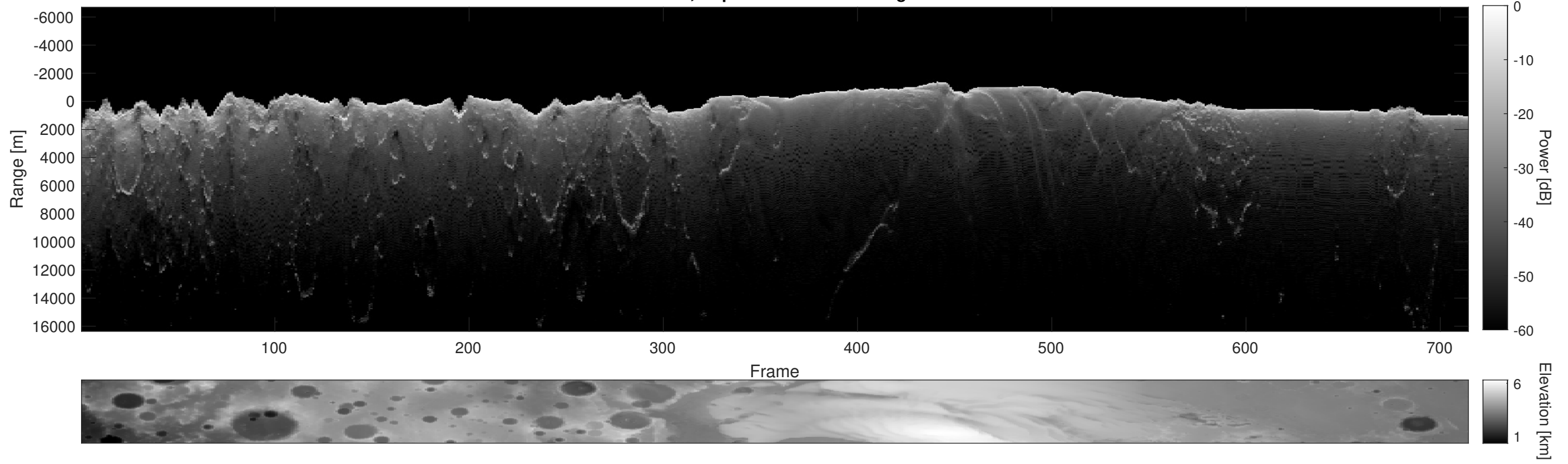
Orbit 6589, Depth-Corrected Cluttergram
