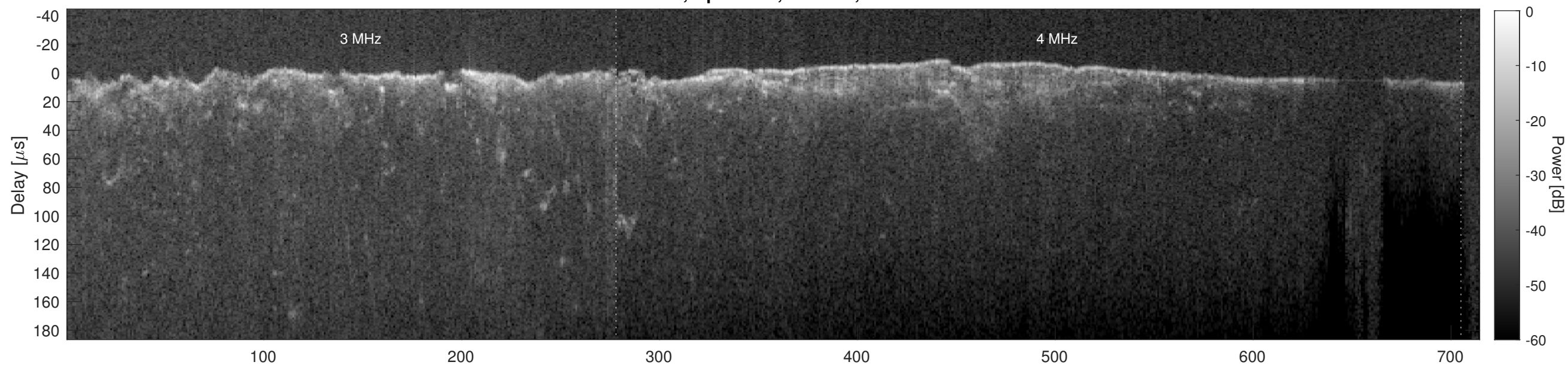
Orbit 6589, Cluttergram
