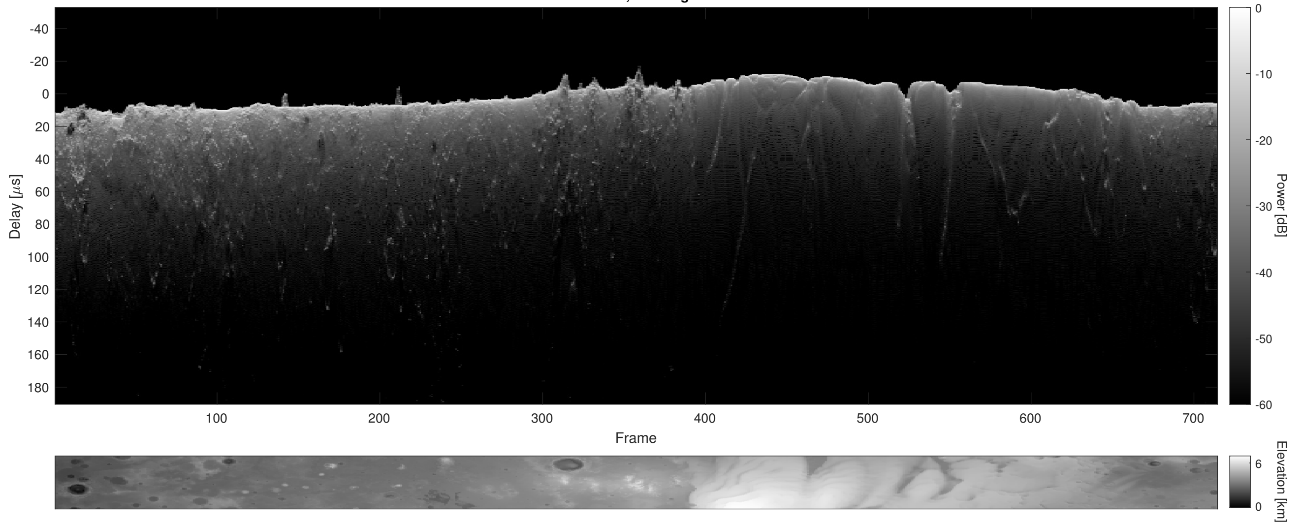
Orbit 6590, Cluttergram
