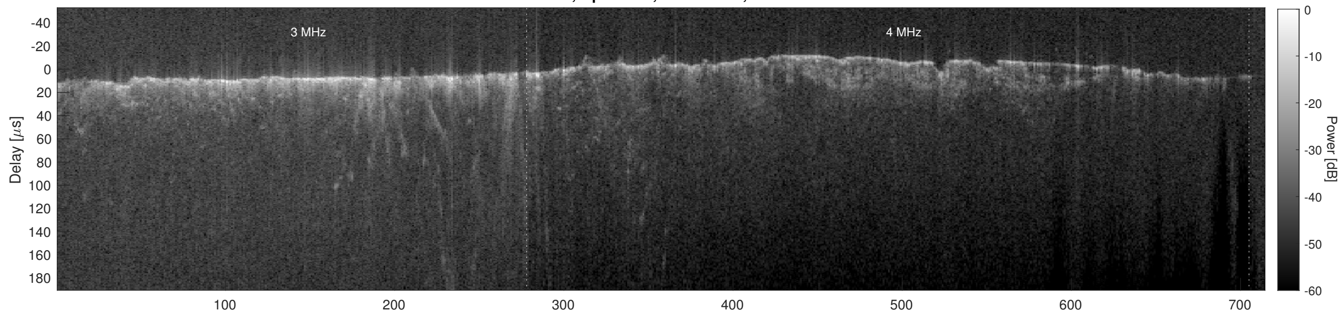
Orbit 6590, Cluttergram
