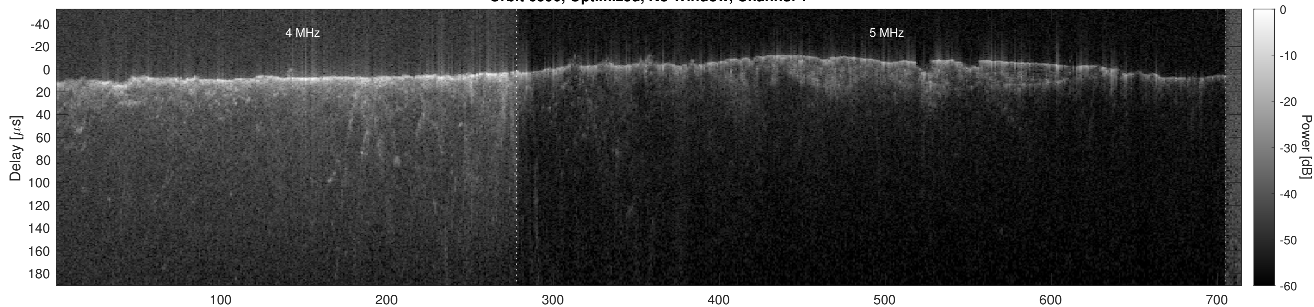
Orbit 6590, Optimized, No Window, Channel 2
