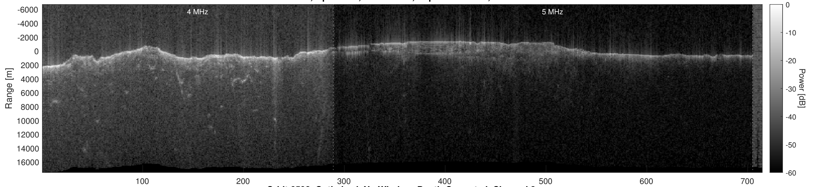
Orbit 6592, Optimized, No Window, Depth-Corrected, Channel 2
