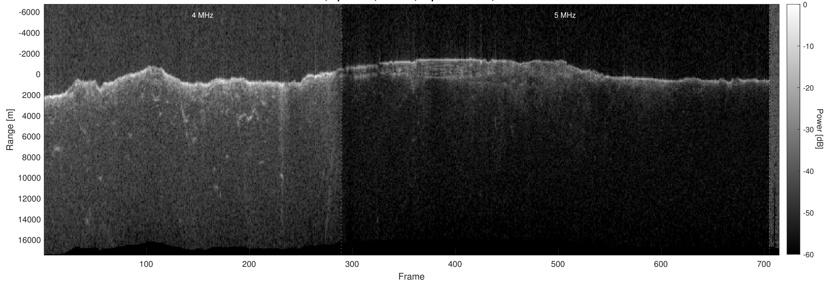
Orbit 6592, Optimized, Window, Depth-Corrected, Channel 2
