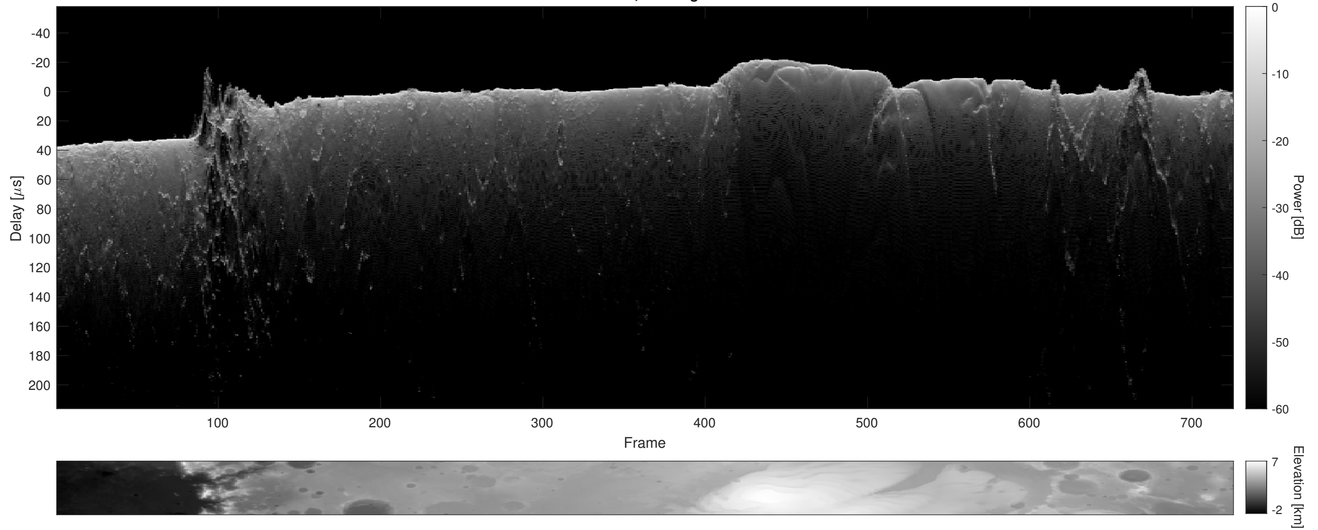
Orbit 6594, Cluttergram
