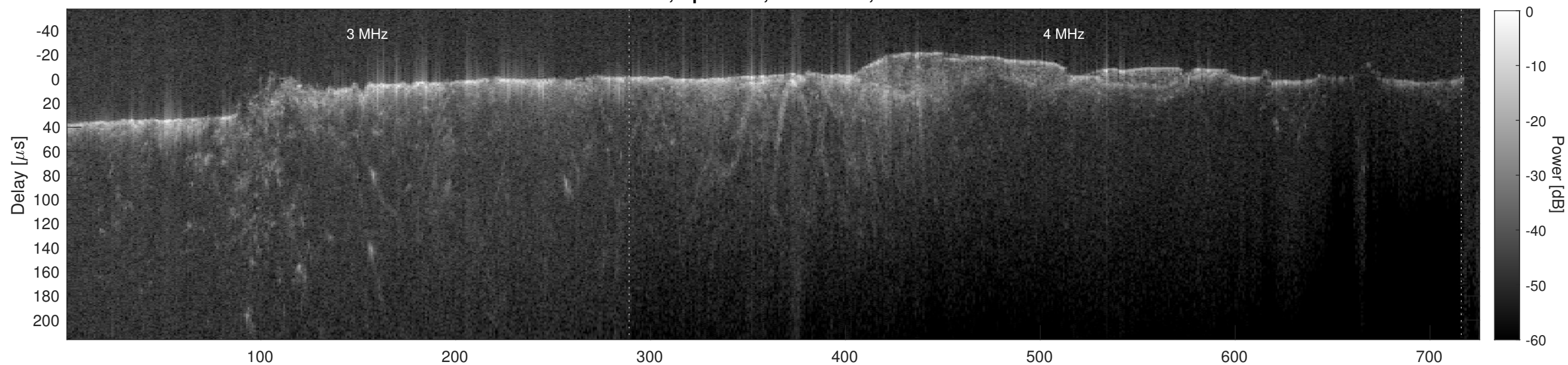
Orbit 6594, Cluttergram
