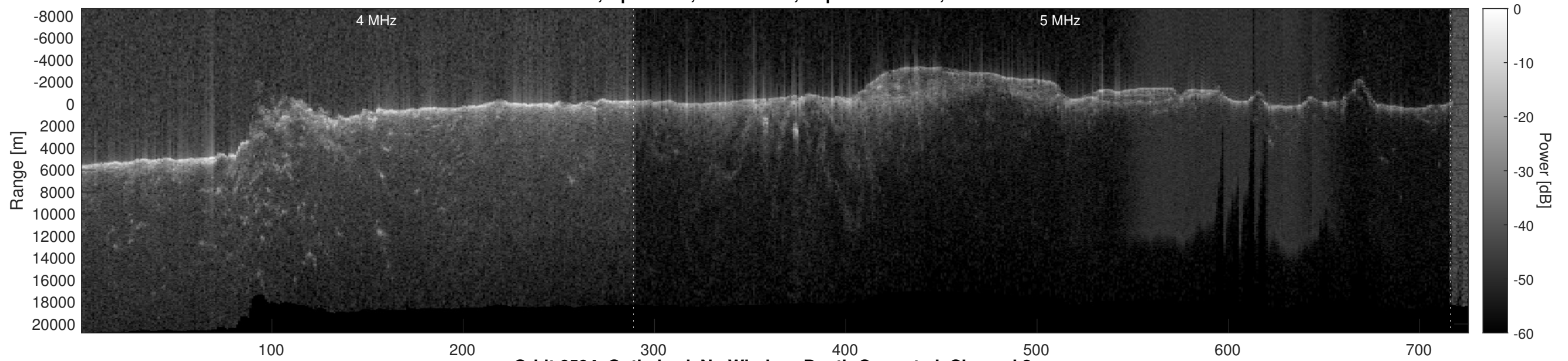
Orbit 6594, Optimized, No Window, Depth-Corrected, Channel 2
