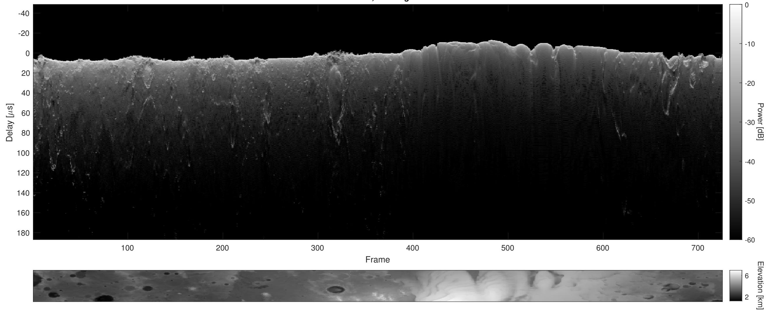
Orbit 6597, Cluttergram
