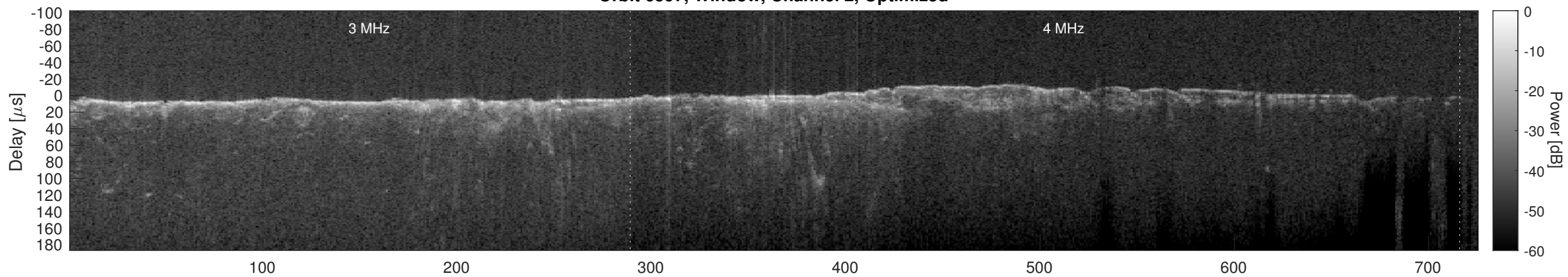
Orbit 6597, Cluttergram
