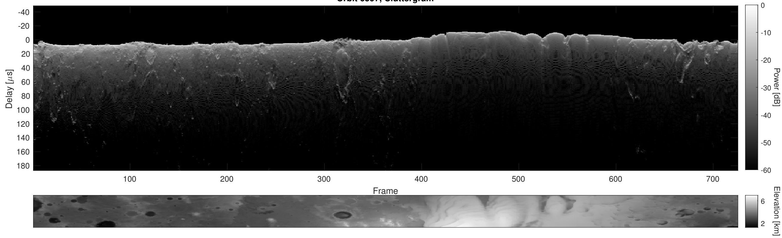
Orbit 6597, Cluttergram
