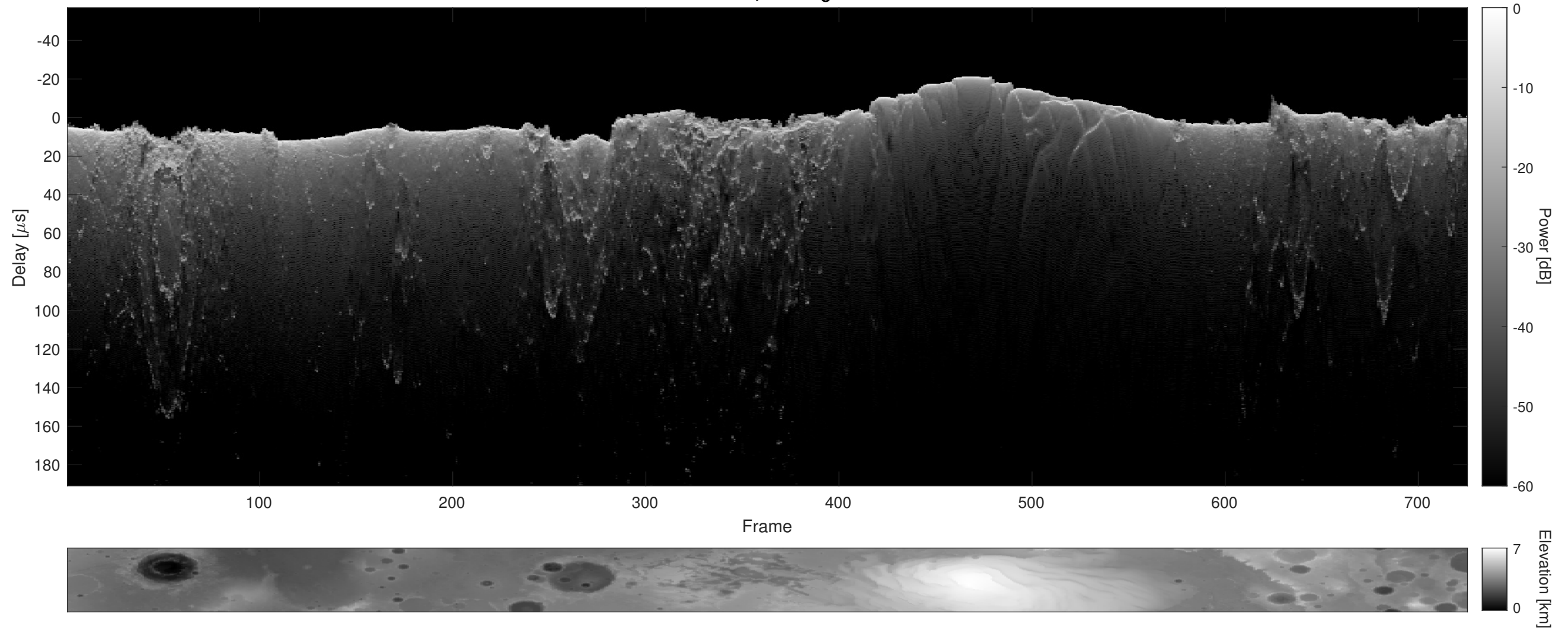
Orbit 6598, Cluttergram
