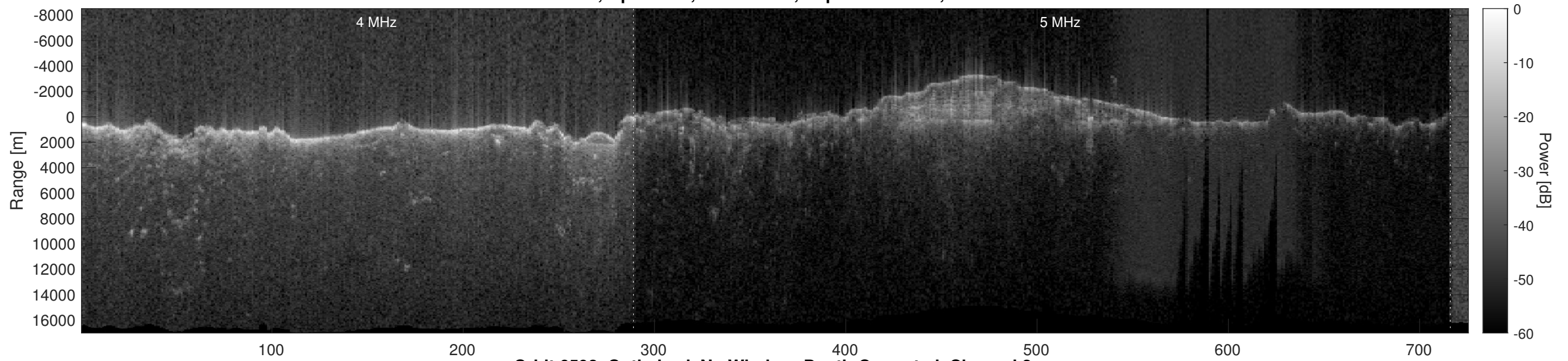
Orbit 6598, Optimized, No Window, Depth-Corrected, Channel 2
