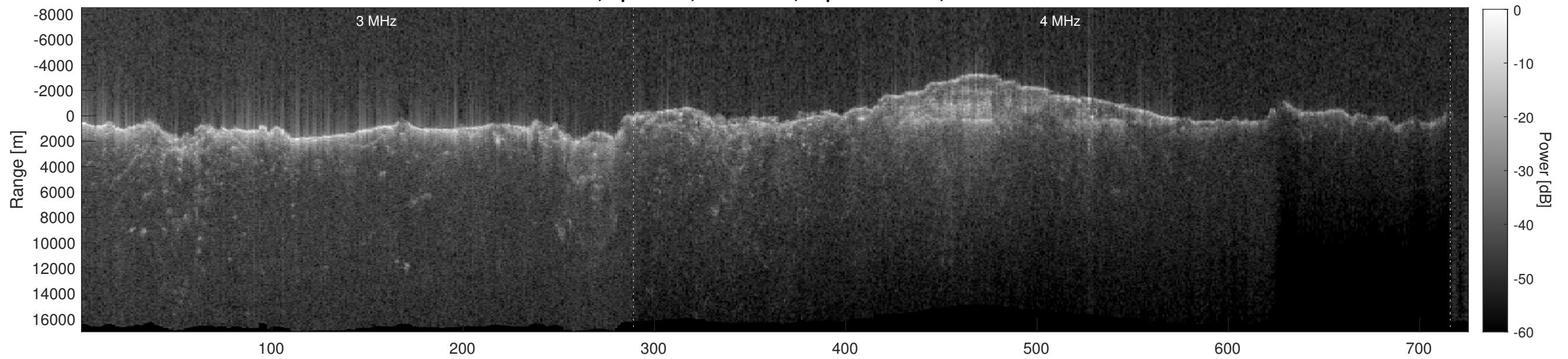
Orbit 6598, Depth-Corrected Cluttergram
