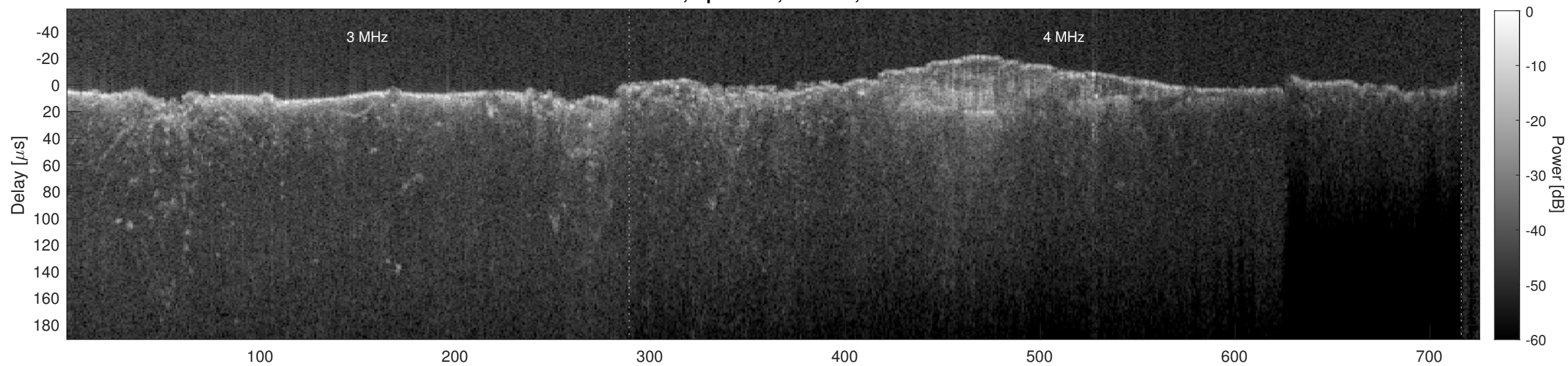
Orbit 6598, Cluttergram
