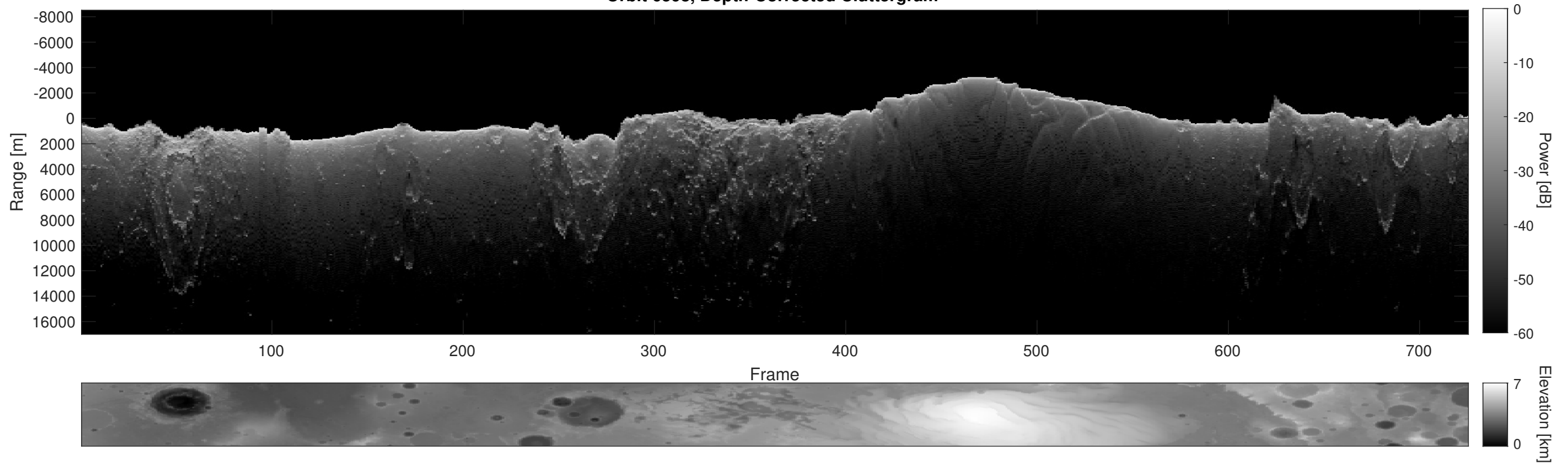
Orbit 6598, Depth-Corrected Cluttergram
