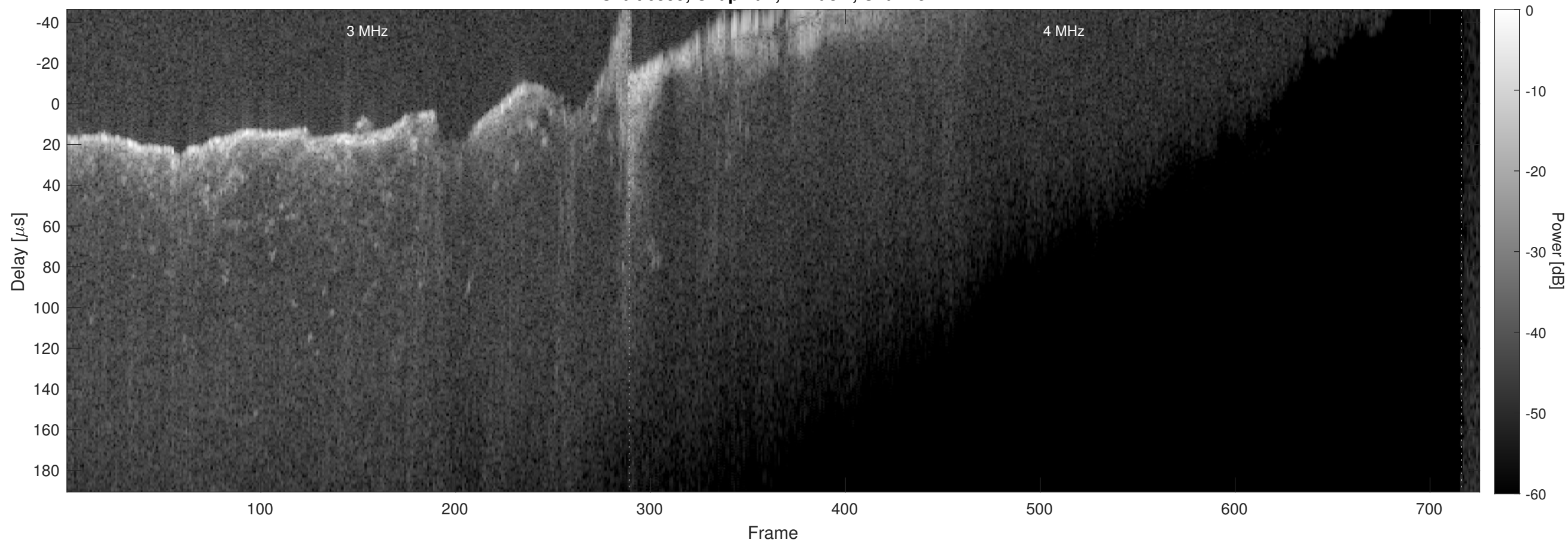
Orbit 6599, Chapman, Window, Channel 2
