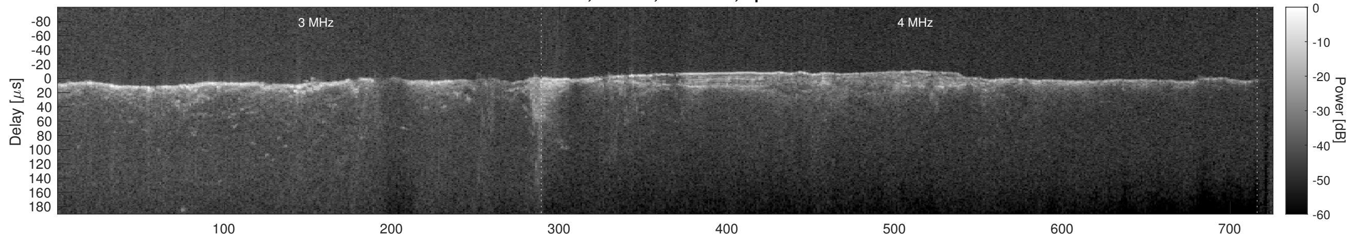
Orbit 6599, Cluttergram
